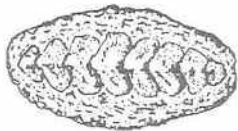
11. Enoplochiton niger
