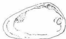
8. Mesodesma donacium
