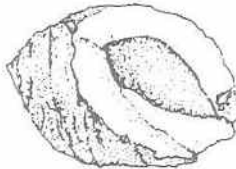
12. Acanthina Sp.
